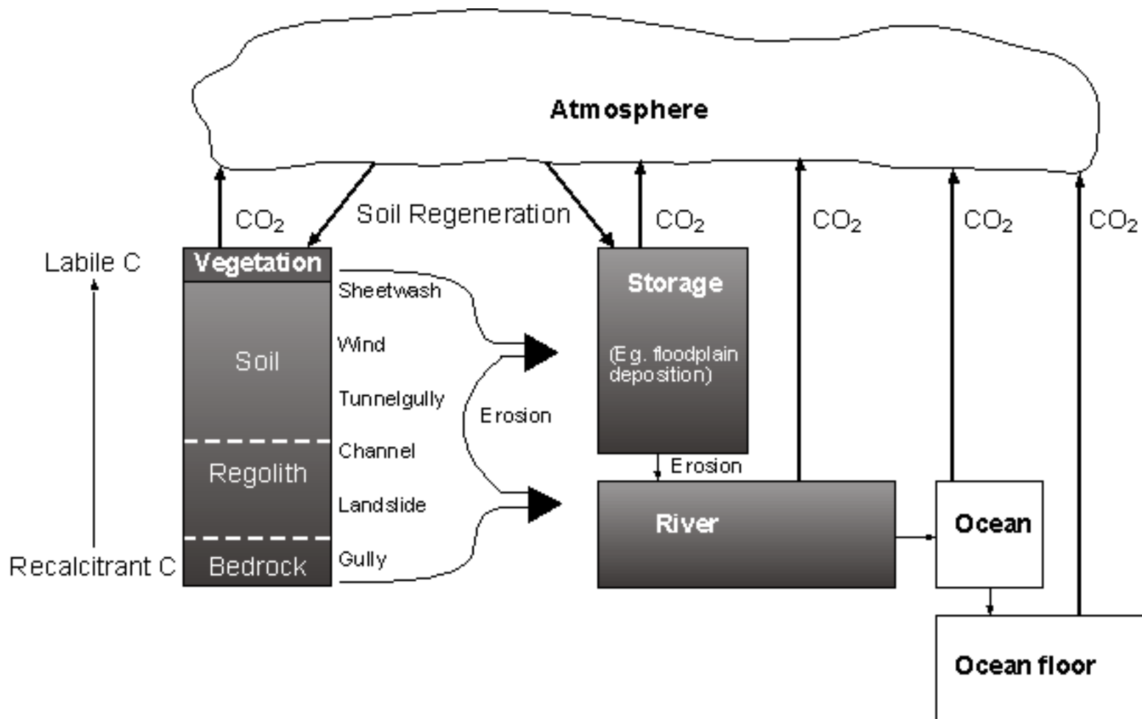
Figure 1: Mass balance approach being used to assess how much eroded C is sequestered annually in land and marine environments and lost annually to the atmosphere as CO 2 . This study is focussed on reporting on potential sources and sinks of erosion-related C in the terrestrial environment. The size of arrows indicating CO 2 fluxes are not related to their magnitude.
